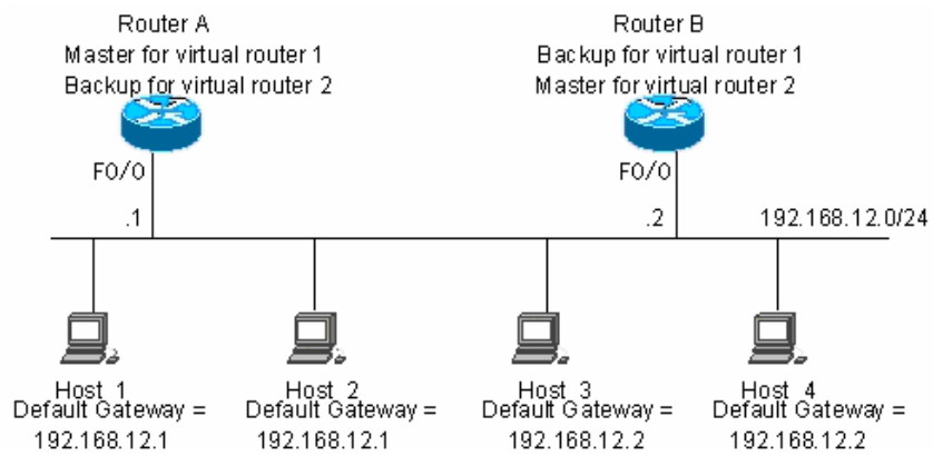
3 VRRP
